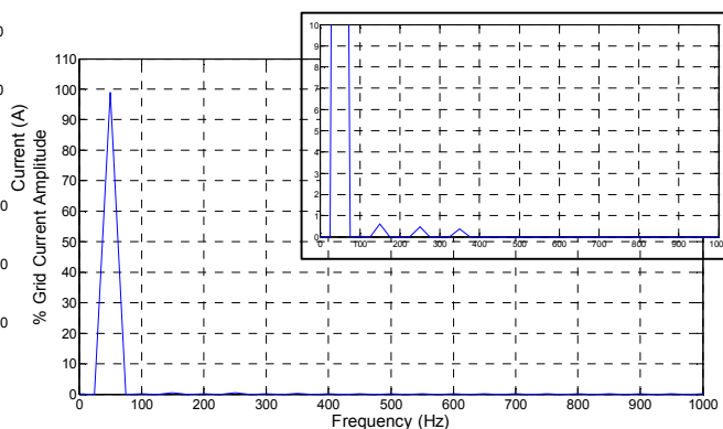
Fig. 13 Harmonic Spectrum of the Grid Current from the Simulation with PR Current Control with Harmonic Compensation
