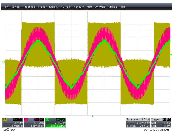
Fig. 15 Inverter Output Voltage (Gold/Yellow Trace), Grid Voltage (Violet Trace) and Grid Current (Green Trace) with a Preset Current of 8A Peak using the PR Controller without Harmonic Compensation
