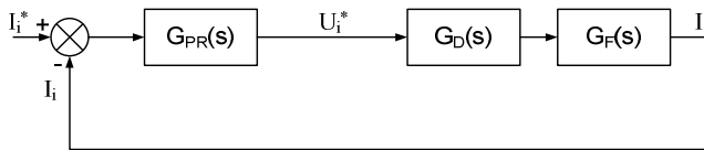
Fig. 2 The PR Current Control
