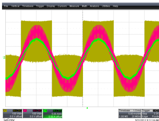
Fig. 16 Inverter Output Voltage (Gold/Yellow Trace), Grid Voltage (Violet Trace), and Grid Current (Green Trace) with a Preset Current of 8A Peak using the PR Controller with 3 rd , 5 th and 7 th Harmonic Compensation
