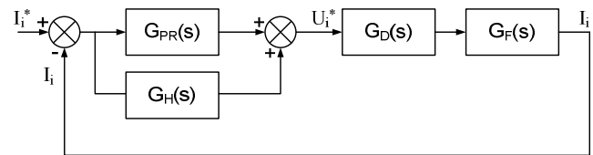
Fig. 3 The PR Current Control with Harmonic Compensators
