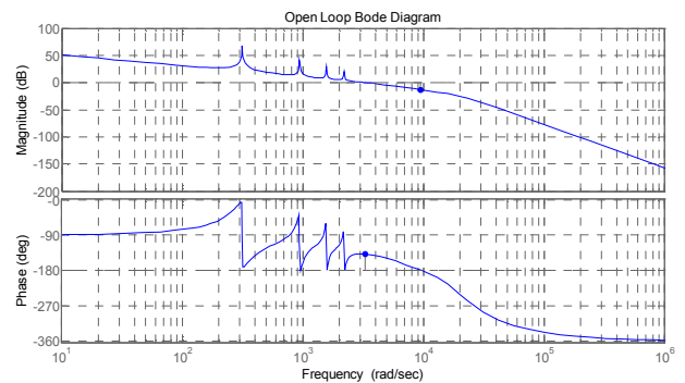
Fig. 8 Open Loop Bode Diagram of the System with the Fundamental PR Controller and the Harmonic Compensators
