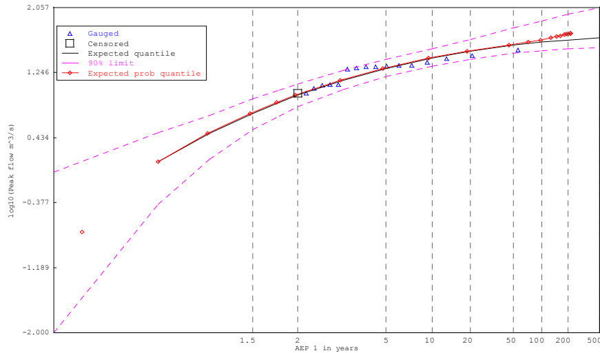
Fig. 8 Fitting of the LP3 distribution to the AM flood data for Station 230204 (17 PILFs censored by MGB test)
