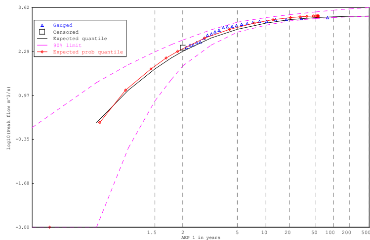
Fig. 3 Flood frequency curve for Station 218005 using LP3 distribution (24 PILFs censored as per MGB test)
