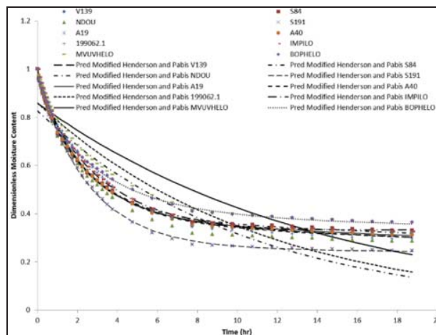
Fig. 9 Comparison between experimental and predicted moisture ratios using Modified Henderson and Pabis model for convective hot air drying of sweet potato slices as a function of drying time at 60°C
