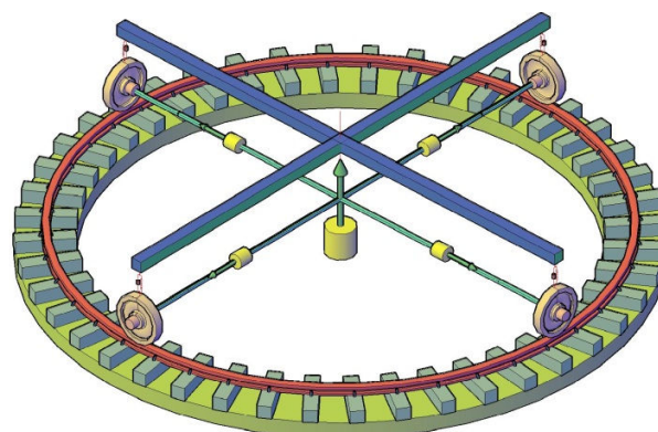
Fig. 1 Schematic view of the new test rig (multiple wheel on single rail track)
