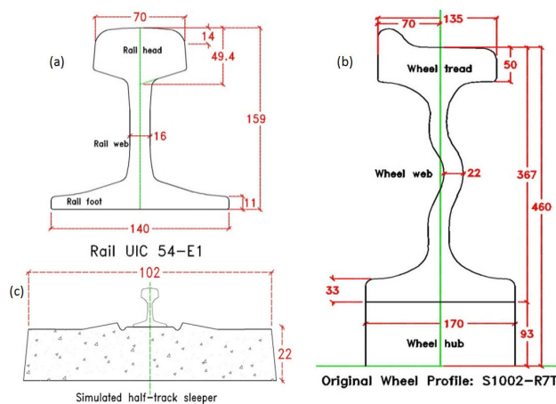
Fig. 2 Actual /full-size components, rail (a), wheel (b), sleeper (c), for normal Dutch railway, all dimensions are in mm
