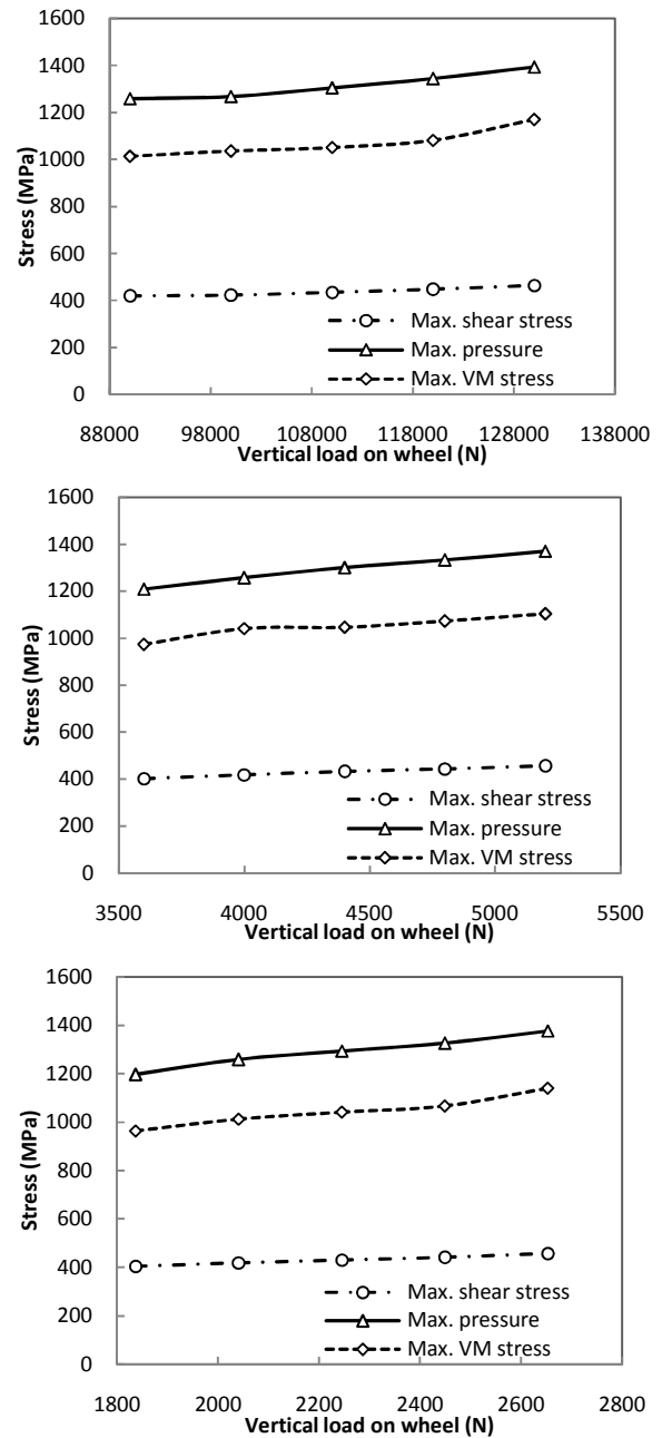
Fig. 9 The results of stress responses in different cases by changing the load levels for (a) Case-1, actual wheel-rail, (b) Case-2, 1/5 scaled test rig, (c) Case-3, 1/7 scaled test rig
