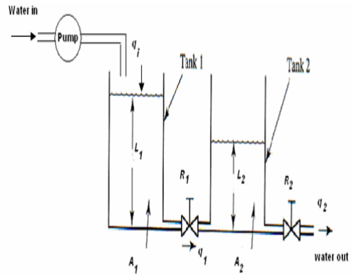
Fig. 6 Dual tank system
