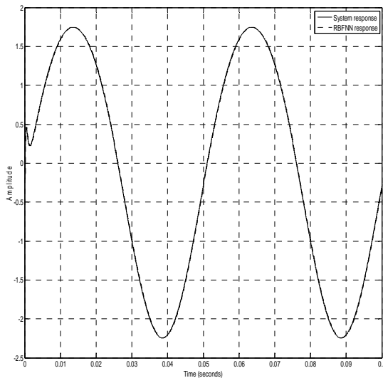
Fig. 13 System output and RBFNN output
