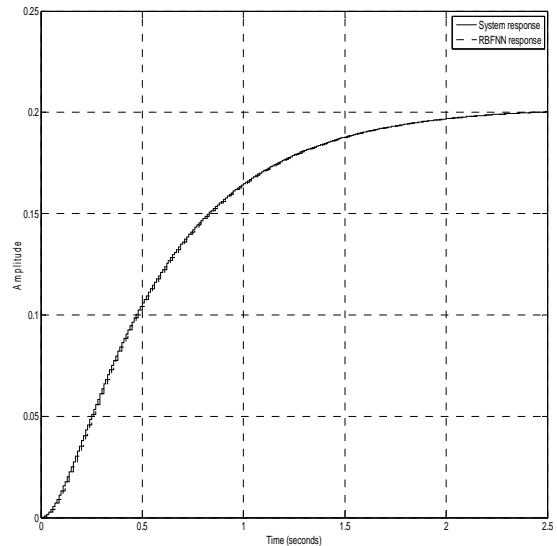
Fig. 11 System output and RBFNN output
