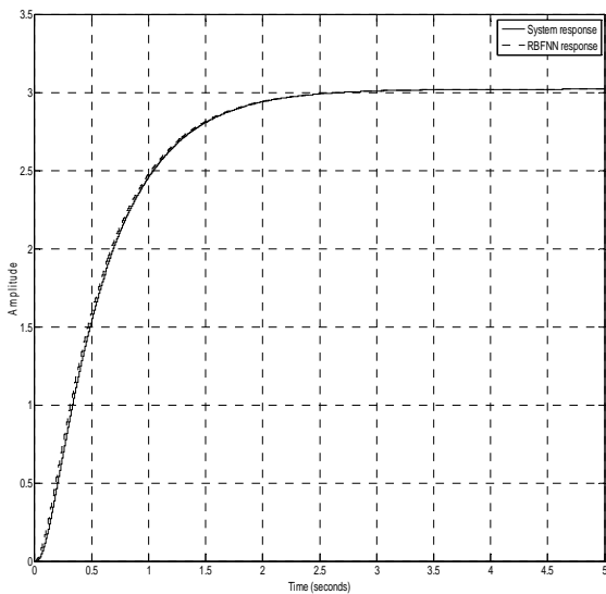
Fig. 9 System output and RBFNN output
