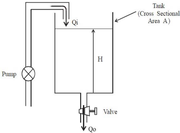
Fig. 8 Single tank system
