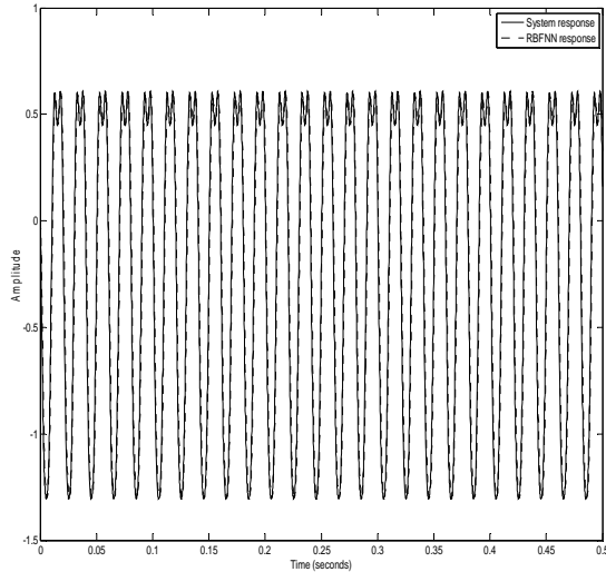
Fig. 12 System output and RBFNN output
