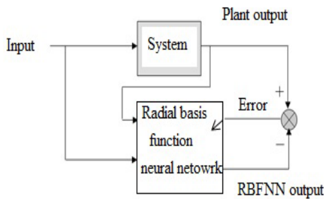
Fig. 5 Series-parallel identification schemes
