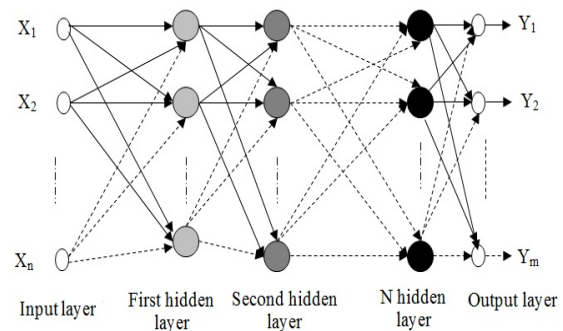
Fig. 2 Multilayer perceptrons diagram
