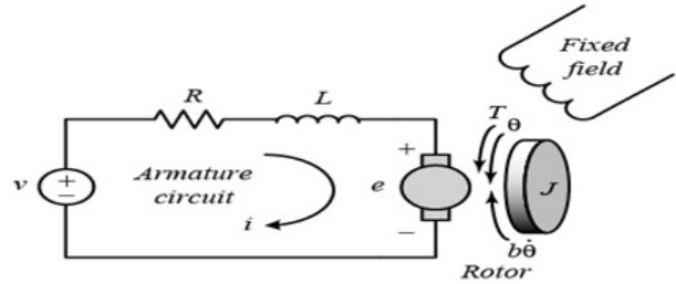
Fig. 10 DC motor system
