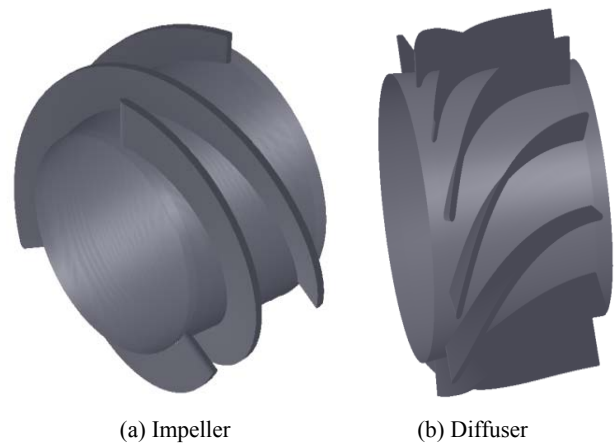
Fig. 2 3D shape of impeller and diffuser for the model pump
