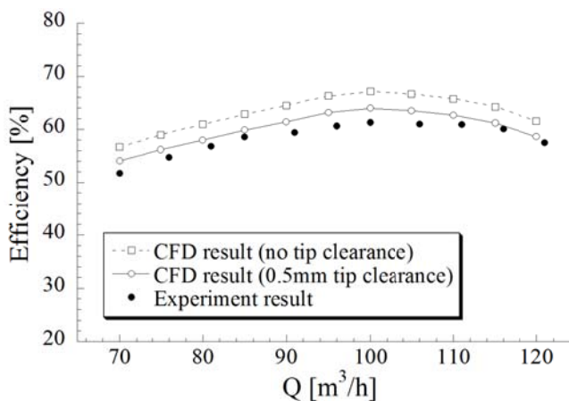
(b) Result of the efficiency difference
