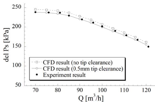
(a) Result of the pressure difference
