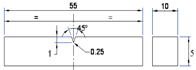
Fig. 2 Dimensions of the impact test specimens with tolerances [ASTM E 23]
