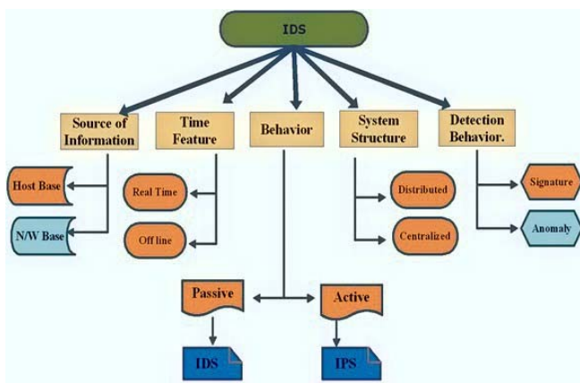
Fig. 1 IDS Types
