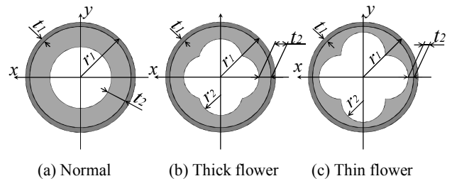
Fig. 4 FEA and experimental objects
