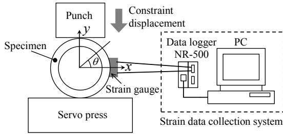
Fig. 9 Diagrammatic illustration of experimental equipment
