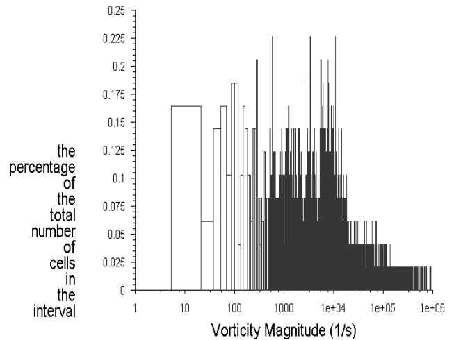
Fig. 9 Vorticity spectrum, (Pipe 2), valve at 45o
