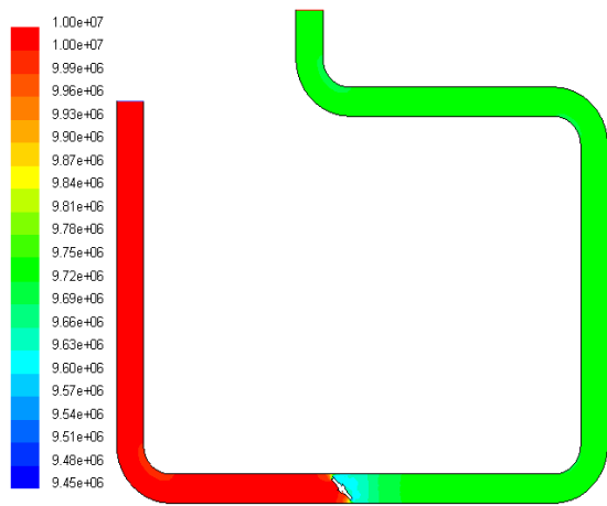
Fig. 6 Static pressure contours (Pipe 1 and Pipe 3), valve at 45°
