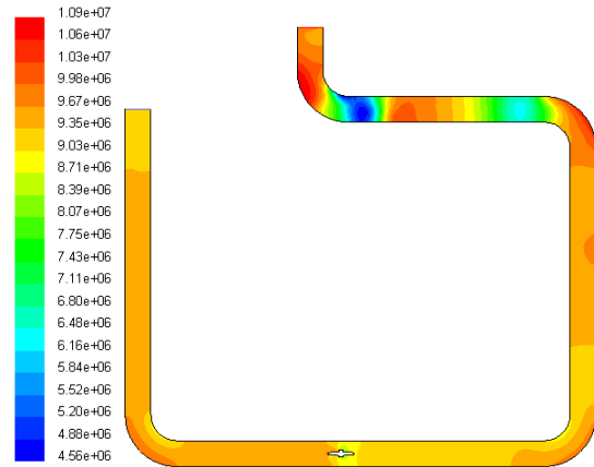
Fig. 4 Static pressure contours, (Pipe 1 and Pipe 3), fully open valve
