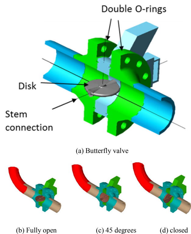
Fig. 1 (a) Butterfly valve and its components (b)-(d) Shaft axis and rotation in relation to elbow
