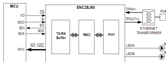
Fig. 3 Ethernet Chip and MCU interconnection
