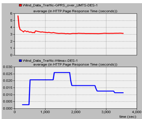
Fig. 13 Average Page response time in HTTP service
