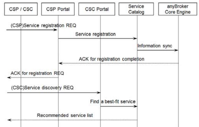
Fig. 8 Sequence diagram for CSP's service registration
