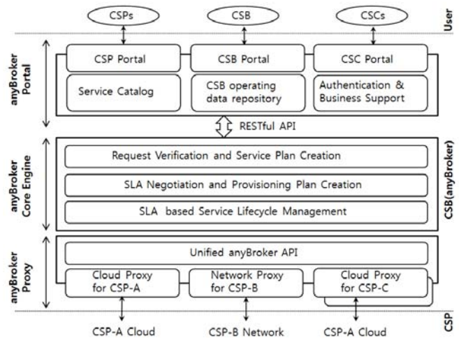
Fig. 1 anyBroker whole architecture
