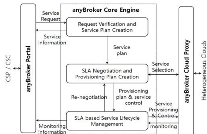
Fig. 4 Component relationship of AnyBroker Engine
