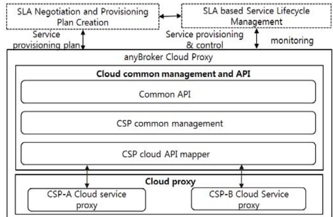
Fig. 7 Operation flow of Cloud proxy
