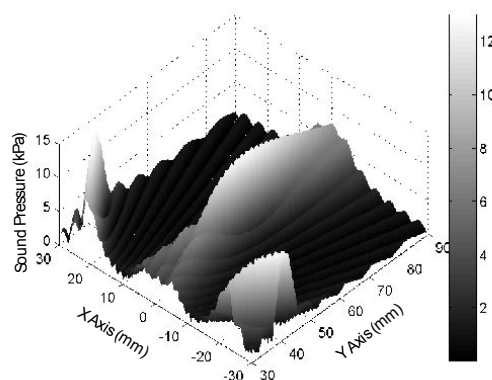
Fig. 4 Ultrasound pressure field simulated in condition of 1MHz frequency, \theta = 2.5^\circ , R = 60 \text{ mm} , P_0 = 0.5 \text{ kPa} and \alpha = 30^\circ
