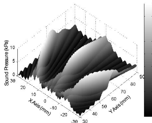
Fig. 5 Ultrasound pressure field simulated in condition of 1MHz frequency, \theta = 3.5^\circ , R = 60 \text{ mm} , P_0 = 0.5 \text{ kPa} and \alpha = 30^\circ
