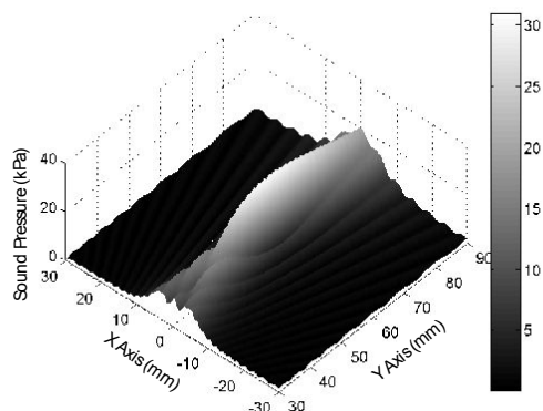
Fig. 3 Ultrasound pressure field simulated in condition of 1MHz frequency, \theta = 1^\circ , R = 60 \text{ mm} , P_0 = 0.5 \text{ kPa} and \alpha = 30^\circ
