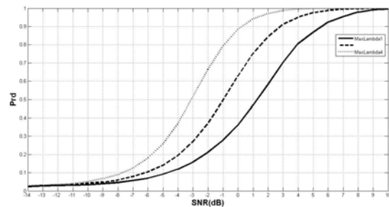
Fig. 8 Detection curves for maxLambda for different number of elements of the antenna array
