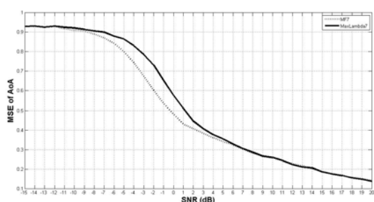
Fig. 11 MSE of AoA for both scenarios
