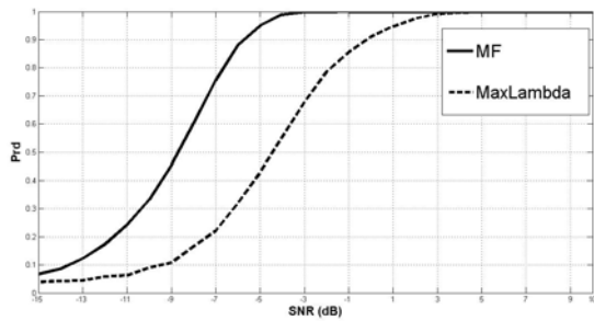
Fig. 4 Detection curves for MF and maxLambda scenarios
