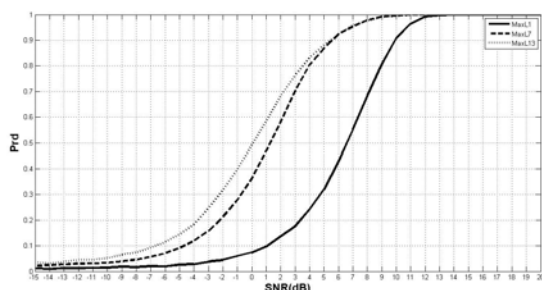
Fig. 6 Detection curves for MaxLambda for different useful signals length
