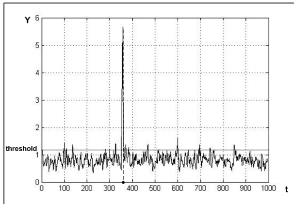
Fig. 2 Principle of AoA estimation
