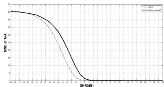
Fig. 14 MSE of ToA for both scenarios
