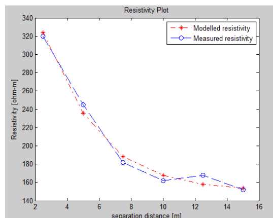
Fig. 10 Comparing the experimental resistivity values of soil with the apparent soil resistivity corresponding to Table V result
