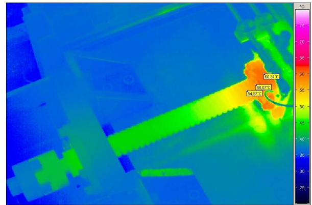
Fig. 17 Thermography image of ball screw drive
