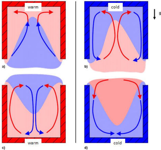
Fig. 11 Convection scenarios for hollow structure
