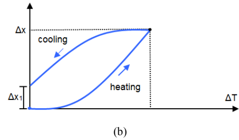
Fig. 20 Linear joint (a) and joint with friction (b)
