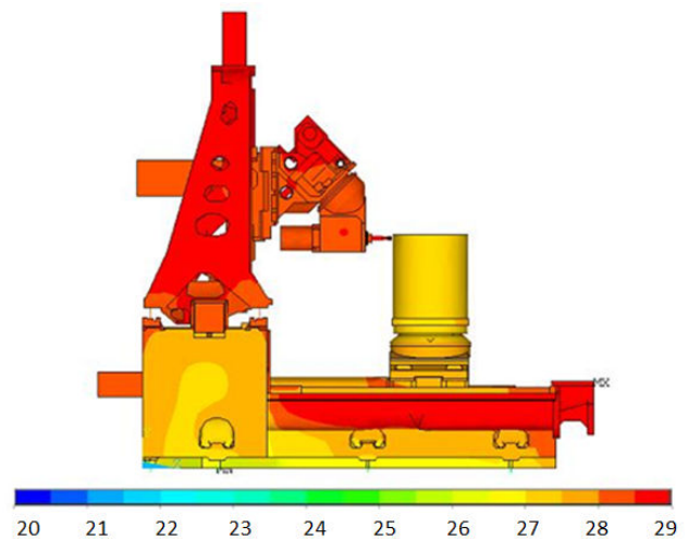
Fig. 21 Thermal field of 5-axis-machining centre
