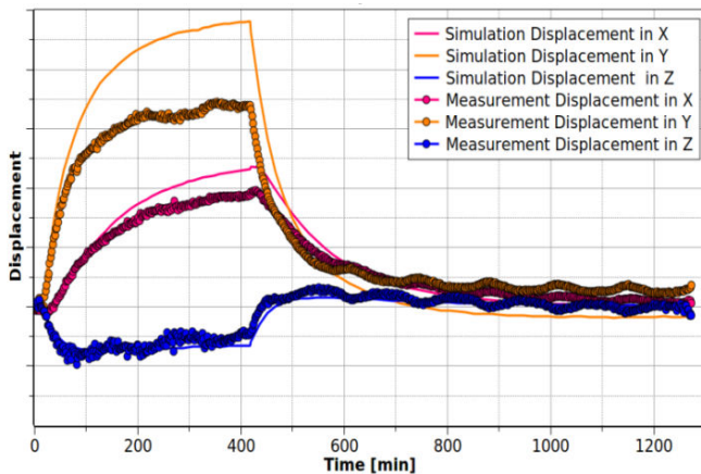
Fig. 19 Measured and simulated displacements
