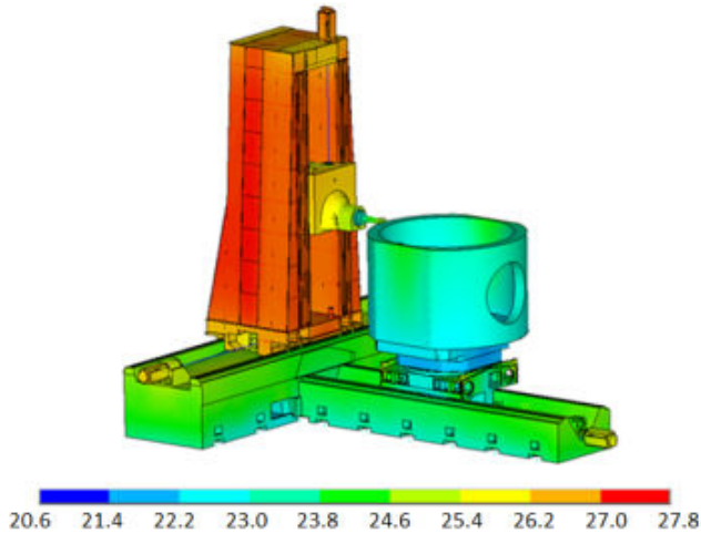
Fig. 22 Thermal field of 4-axis-machining centre
