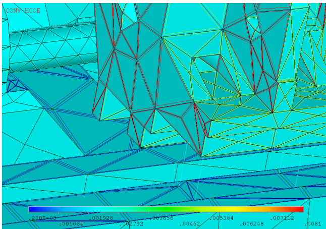
Fig. 8 Heat transfer coefficients of element surfaces
