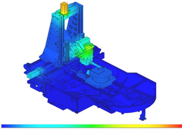
Fig. 18 Temperature field in °C (loadcase 7)
