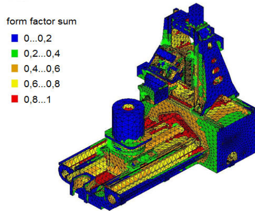
Fig. 13 Form factor sums on element surfaces
