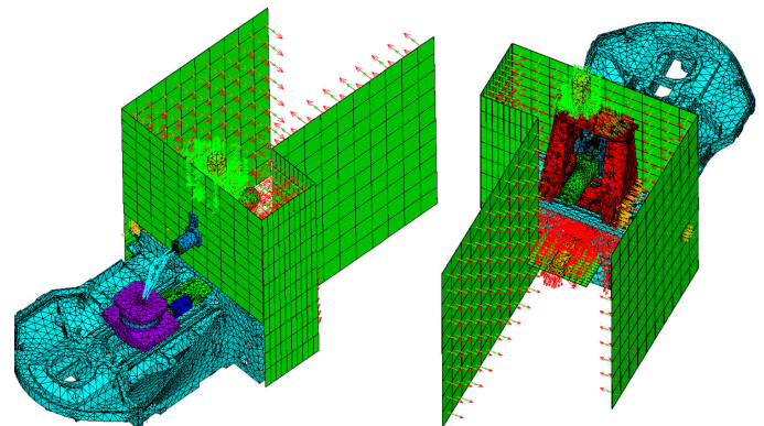
Fig. 14 Heat transfer by radiation with blockades
