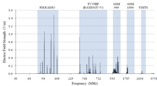
Fig. 6 Instantaneous spectrum
