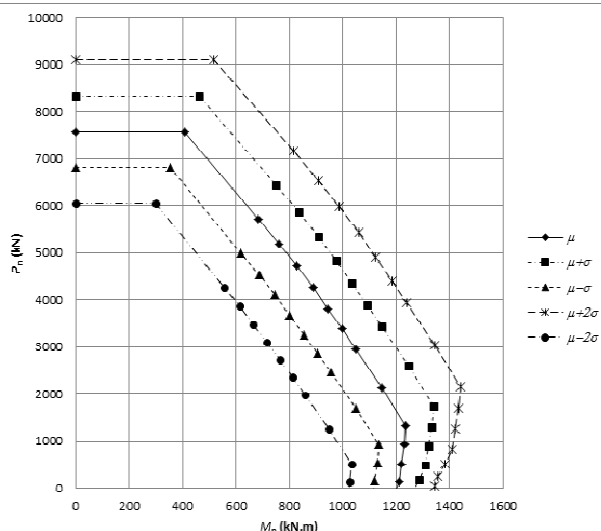
Fig. 5 Interaction diagram for column C1
