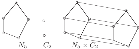
Fig. 2. The direct product N_5 \times C_2
