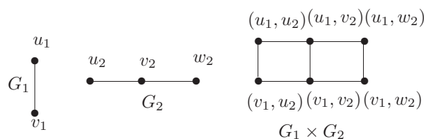
Fig. 1. The product of two graphs
