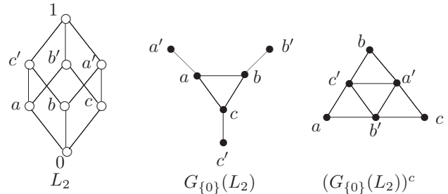
Fig. 4. Zero divisor graph and its complement both are connected
