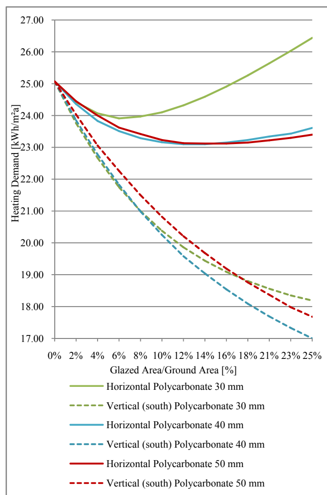
Fig. 8 Heat. demand \theta_i = 17^\circ\text{C} , night/weekend-setback, internal gains
