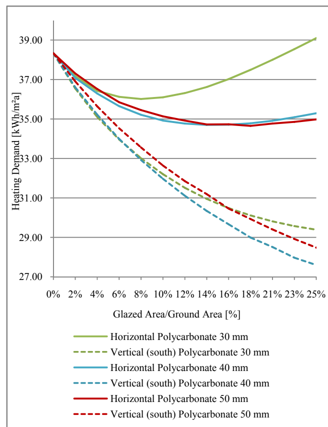
Fig. 9 Heat. demand \theta_i = 20^\circ\text{C} , night/weekend-setback, internal gains
