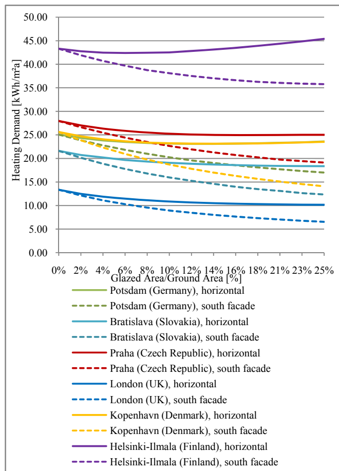
Fig. 10 Heating demand for different climates, 40 mm polycarbonate, \theta_i = 17^\circ\text{C} (setback), internal gains
