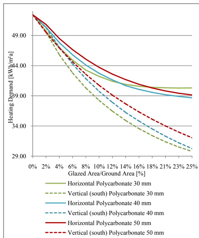
Fig. 7 Heating demand dependent on the glazing area, \theta_i = 12^\circ\text{C}
