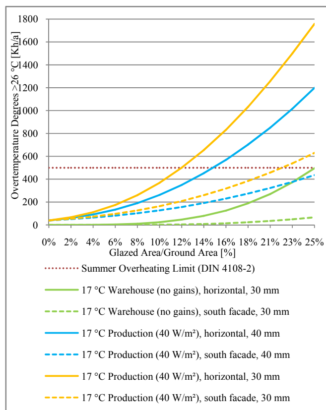
Fig. 11 Summer overheating (DIN 4108-2), 40 mm polycarbonate
