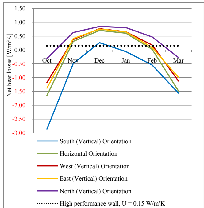
Fig. 5 Performances for different orientations, 30 mm PC, \theta_i = 20^{\circ}\text{C}
