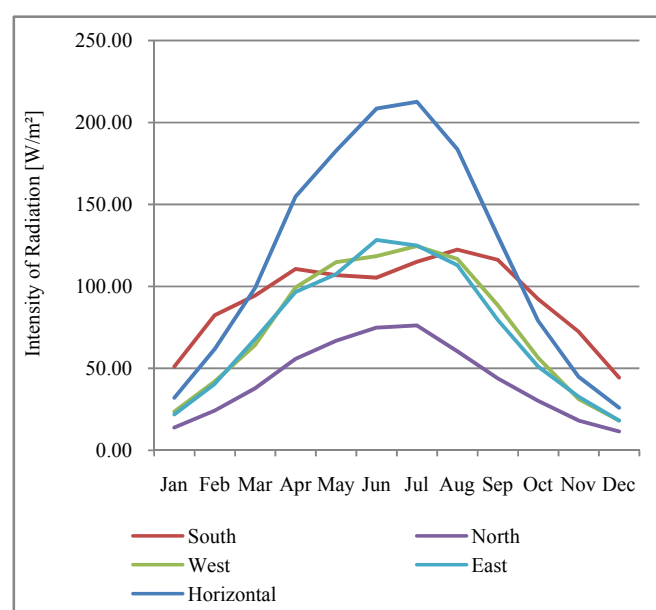
Fig. 1 Intensity of radiation for different orientations in Potsdam
