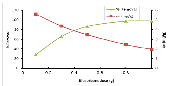
Fig. 2 Effect of BPAC dose on manganese biosorption
