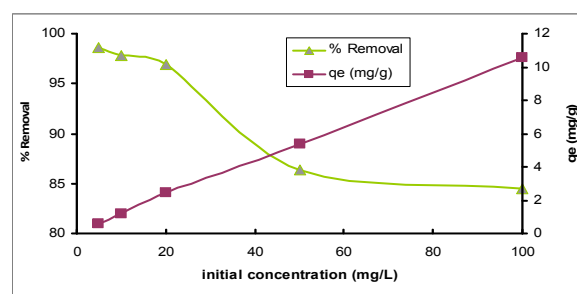
Fig. 3 Effect of initial metal ion concentration on manganese biosorption by BPAC
