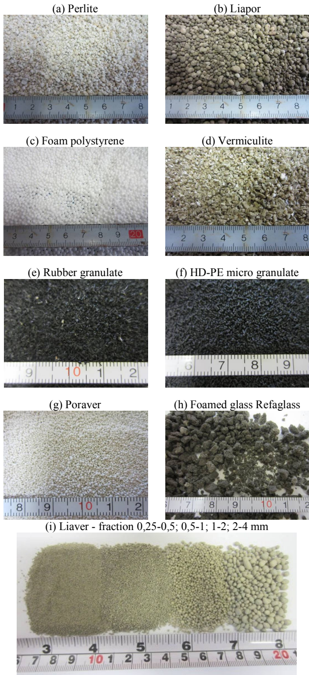
Fig. 1 The illustration of the light fillers
