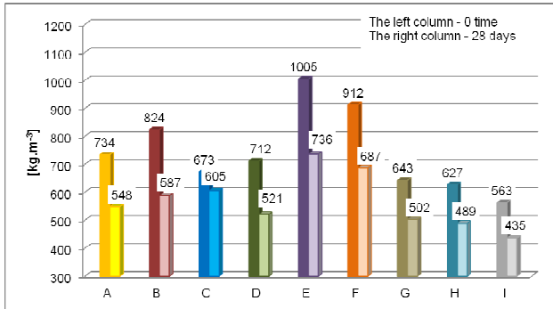
Fig. 3 The evaluation of bulk density
