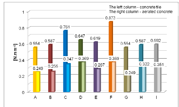
Fig. 6 The evaluation of adhesive strength on substrates
