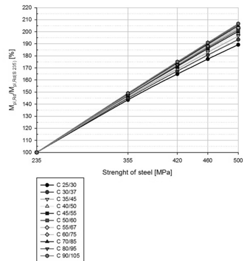
Fig. 4 The relation between the ratio of M_{pl,Rd}/M_{pl,Rd}(C25/30) and strength of steel for composite beams with C
