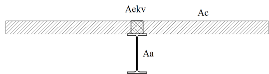
Fig. 8 The effective equivalent cross-section
