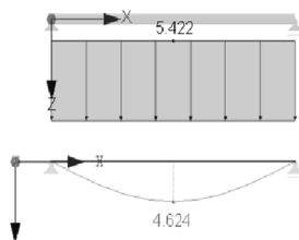
Fig. 12 The deformation caused by self-weight
