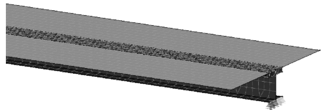
Fig. 14 Numerical model using contact surfaces
