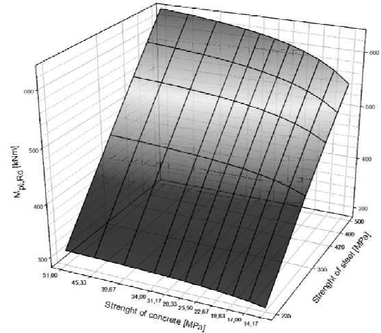
Fig. 2 The spatial relation between plastic resistance and strength of concrete and strength of steel for composite beams with C
