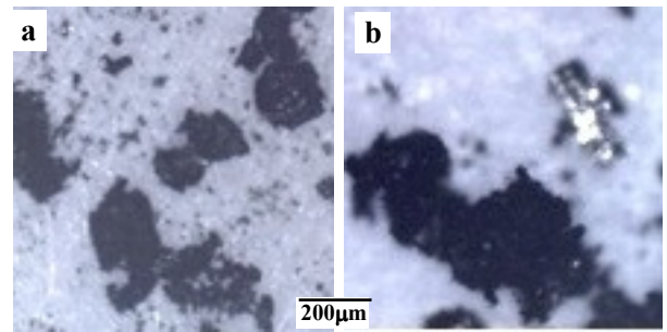
Fig. 6 Wear debris collected from wear test at 1.4 MPa (20N) applied pressure and sliding distance of 4200m for (a) Block, (b) Piston
