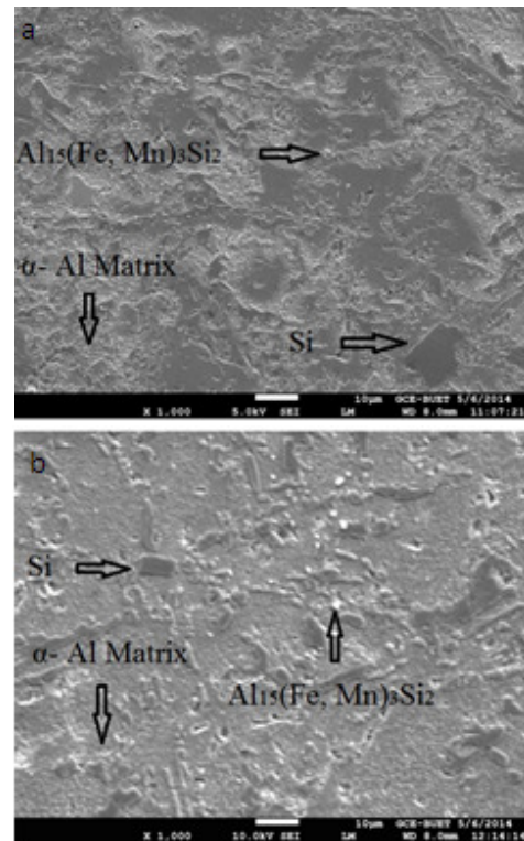
Fig. 7 SEM micrographs of as-received Al-Si (a) block and (b) piston
