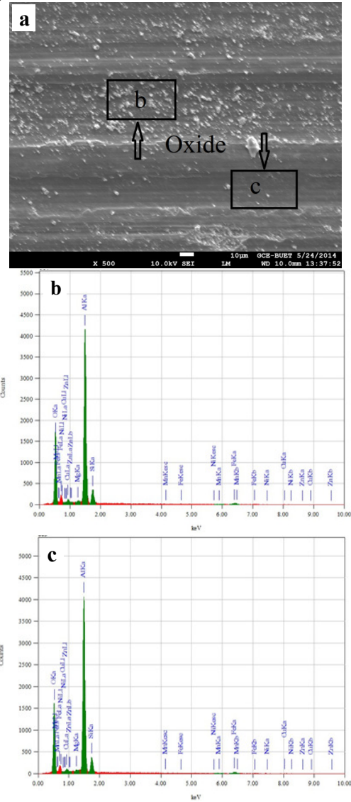
Fig. 9 SEM images of worn surfaces of aluminium engine piston after wear at 1.4 MPa applied pressure and sliding distance of 4200m
