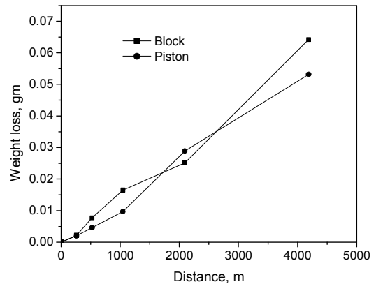
Fig. 2 Variation of weight loss (gm) with the variation of sliding distance (m) at applied pressure of 1.4 MPa (Load 20N) and sliding velocity 0.29 \text{ ms}^{-1}
