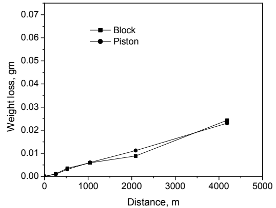
Fig. 1 Variation of weight loss (gm) with the variation of sliding distance (m) at applied pressure of 0.30MPa (Load 5N) and sliding velocity 0.29 \text{ ms}^{-1}
