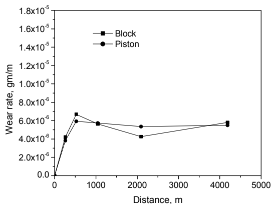
Fig. 3 Variation of wear rate (gm/m) with the variation of sliding distance (m) at applied pressure of 0.30 MPa (Load 5N) and sliding velocity 0.29 ms -1
