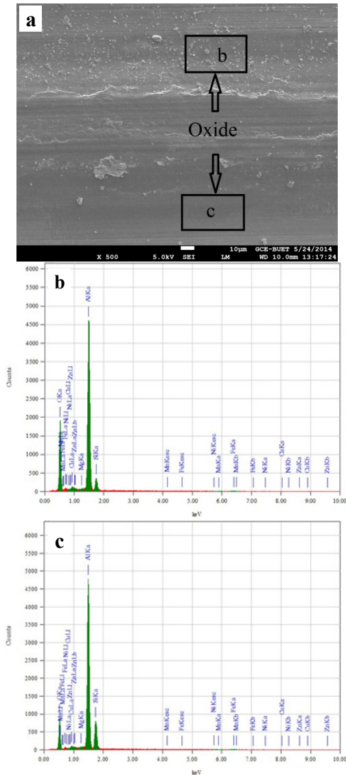
Fig. 8 SEM images of worn surfaces of aluminium engine block after wear at 1.4 MPa applied pressure and sliding distance of 4200m
