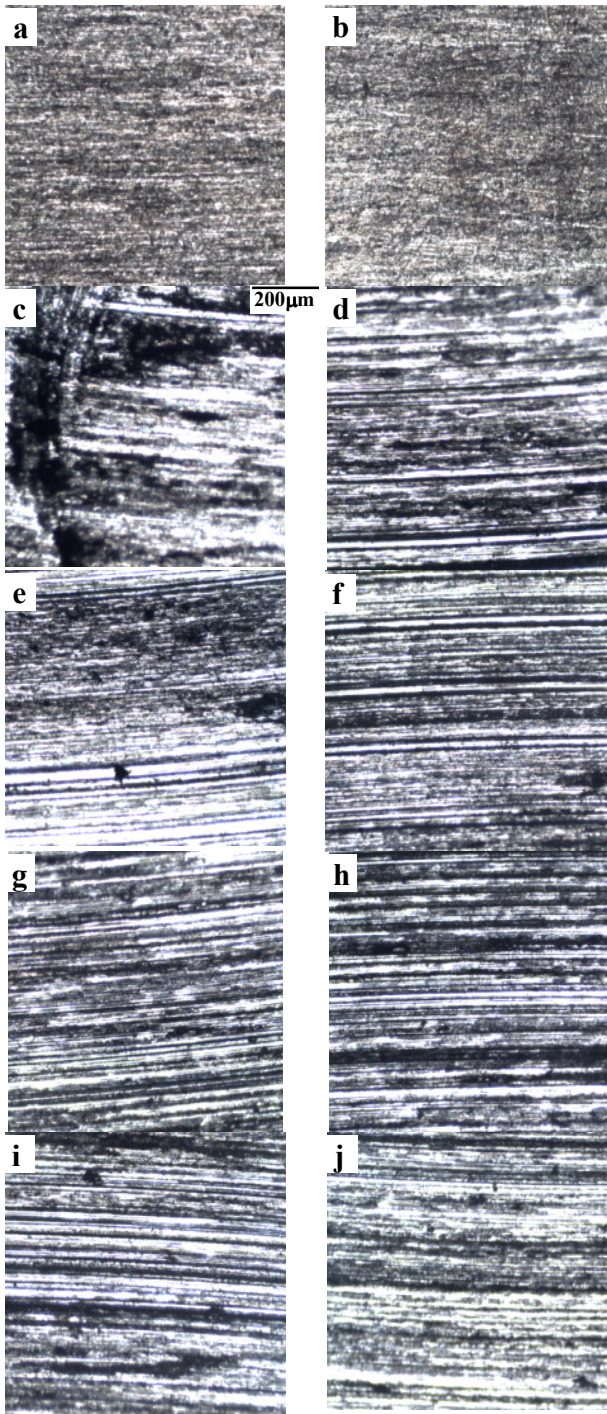
Fig. 5 Optical micrograph of worn surfaces before wear (a) block, (b) piston, after wear at applied pressure of 0.30MPa for 15 min (c) block, (d) piston, for 4 hours (e) block, (f) piston, at applied pressure of 1.40MPa for 15 min (g) block, (h) piston and for 4 hours (i) block (j) piston
