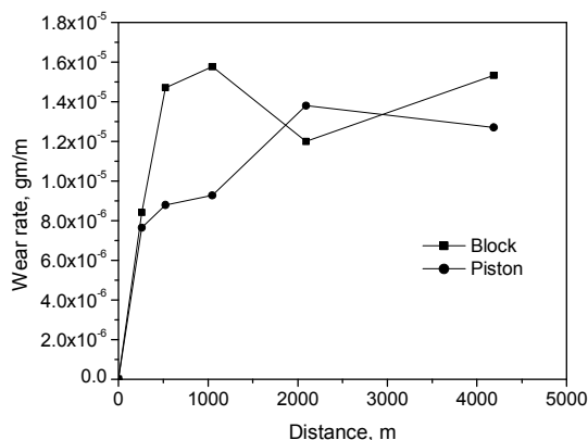
Fig. 4 Variation of wear rate (gm/m) with the variation of sliding distance (m) at applied pressure of 1.4 MPa (Load 20N) and sliding velocity 0.29 ms -1
