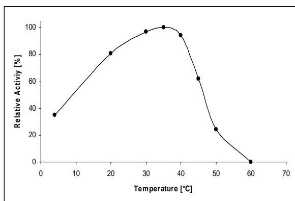
Fig. 2 Effect of temperature on poppy PPO activity
