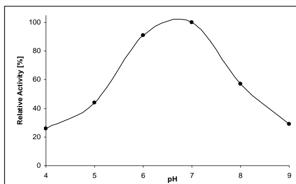
Fig. 1 Effect of pH on poppy PPO activity
