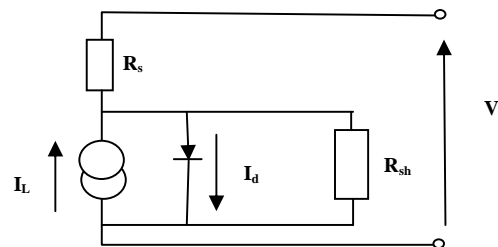
Fig. 1 Equivalent circuit of solar cell (1-diode model)
