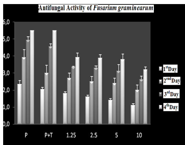
Fig. 4 Antifungal Activity of Fusarium graminearum
