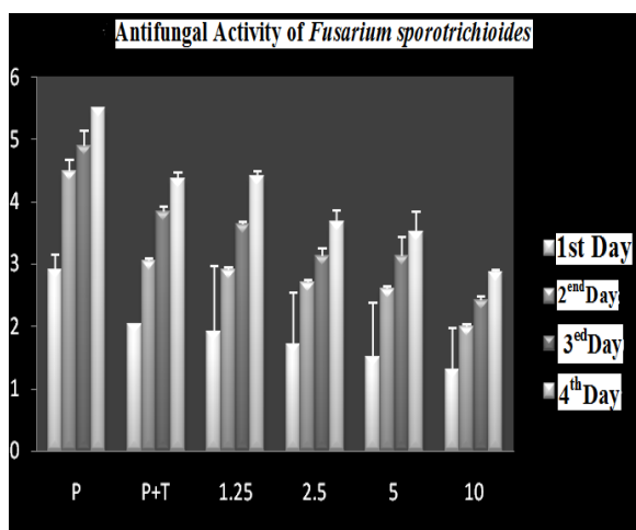
Fig. 3 Antifungal Activity of Fusarium sporotrichioides
