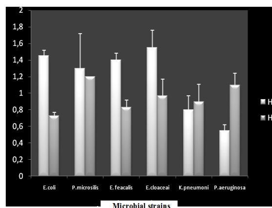
Fig. 2 Antimicrobial activity of HE Eucalyptus camendulensis
