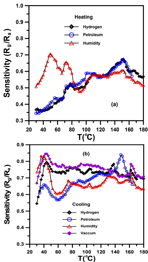
Fig. 8 Sensitivity as a function of temperature for (a) heating and (b) cooling of \text{Na}_{0.1}\text{V}_2\text{O}_5 \cdot n\text{H}_2\text{O} nanocrystalline film at different gases
