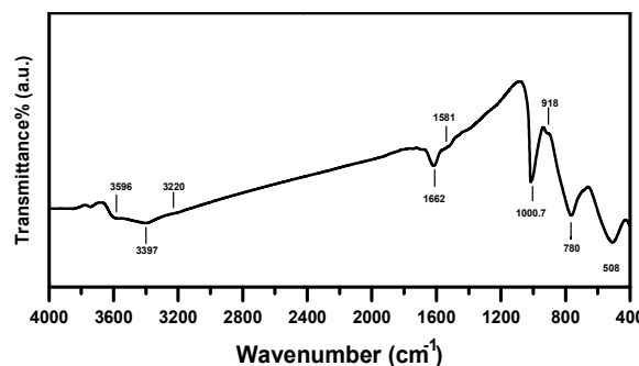
Fig. 5 IR spectra for \text{Na}_{0.1}\text{V}_2\text{O}_5.n\text{H}_2\text{O} nanocrystalline film
