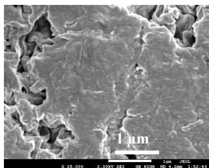
Fig. 4 SEM image for \text{Na}_{0.1}\text{V}_2\text{O}_5.n\text{H}_2\text{O} nanocrystalline film
