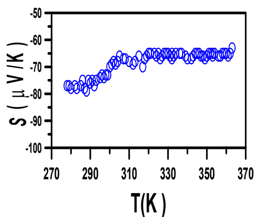
Fig. 7 Thermoelectric power(S) as a function of temperature for \text{Na}_{0.1}\text{V}_2\text{O}_5 \cdot n\text{H}_2\text{O} nanocrystalline film
