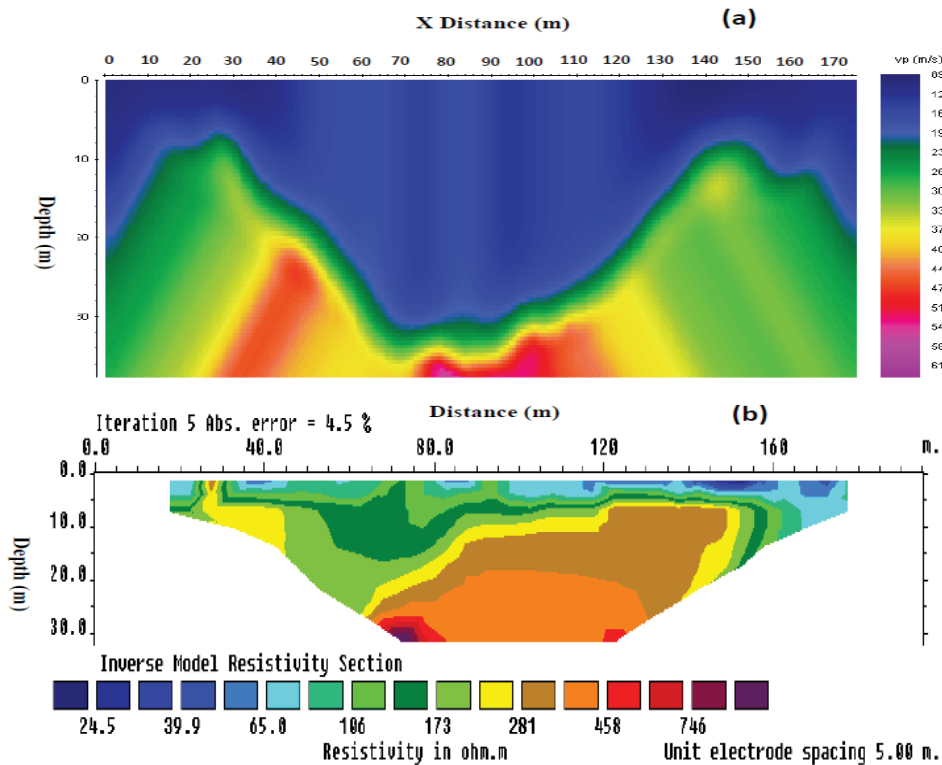
Fig. 4 (a) Third seismic refraction tomography model taken 100 m away from the first profile, (b) Third resistivity tomography model taken 100m away from the first profile
