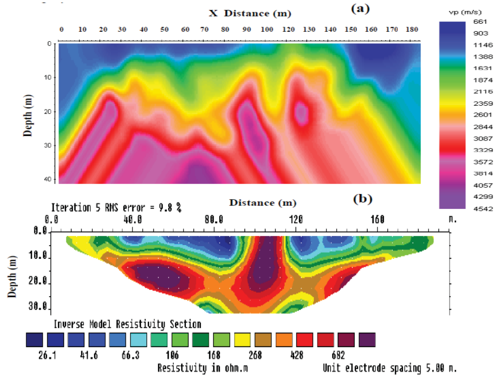
Fig. 2 (a) Seismic refraction tomography model taken in the vicinity of an outcrop across stream channel, (b) First resistivity tomography model taken in the vicinity of an outcrop across stream channel
