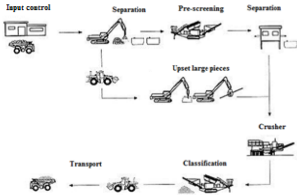
Fig. 1 Basic steps of the recycling process [9]
