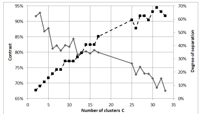
Fig. 5 Contrast (solid line, left axis) and degree of separation (dashed line, right axis) vs number of clusters in the clusterization
