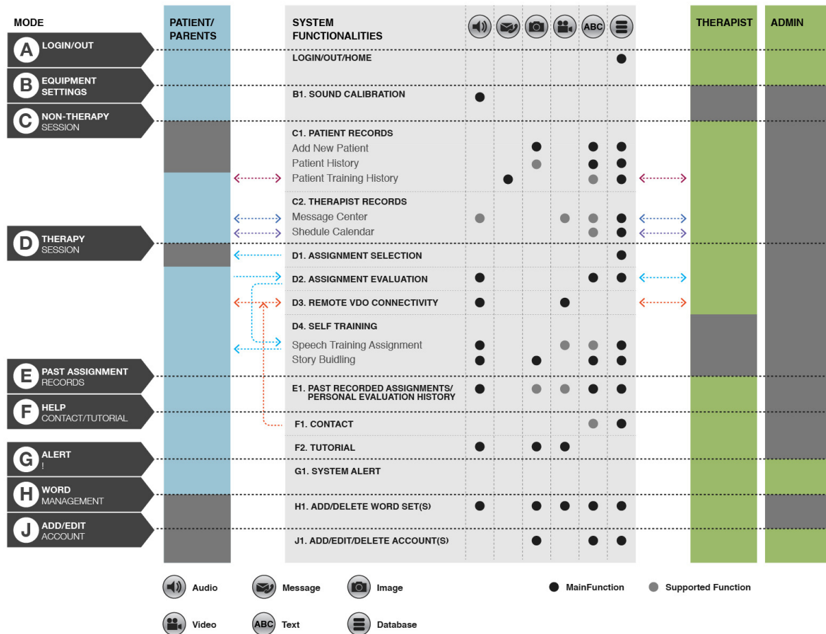
Fig. 2 System Functionalities and Enhancements
