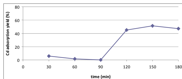
Fig. 7 \text{Cd}^{+2} adsorption yield depending upon time for optimum conditions by using Seyitomer fly ash (with diatomite and molasses)
