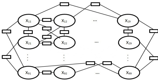
Fig. 3 Parts of the consistency network used in our CSP formulation of Sudoku puzzles.
