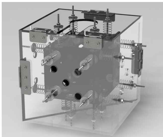
Fig. 2 Mechanical Force Gauge image (by Solid Works)
