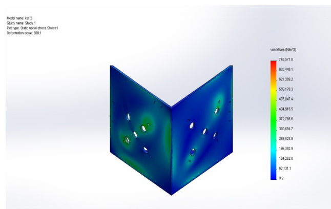
Fig. 3 (c) The outer skin stresses
