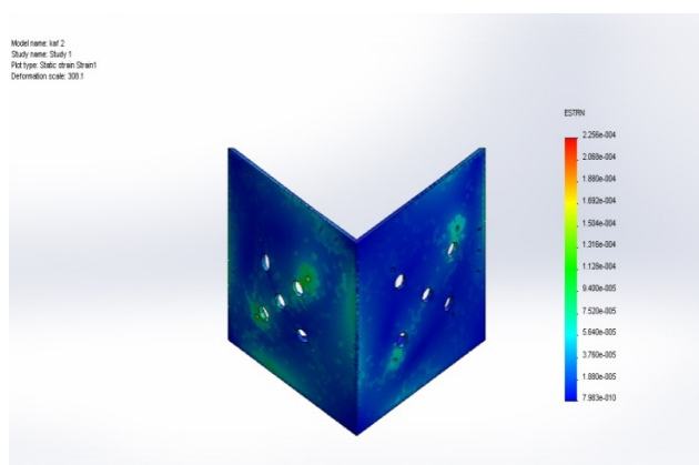
Fig. 3 (a) The outer skin displacement
