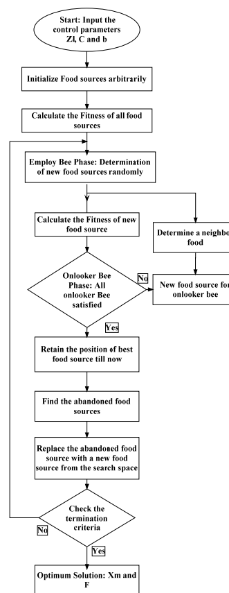
Fig. 2 Flowchart of ABC
