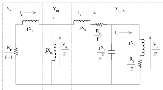
Fig. 1 Per phase equivalent circuit of SEIG
