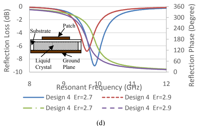
Fig.2 Reflection loss and reflection phase curves for different designs depending on the volume of LC used, (a) Design 1: LC under full patch, (b) Design 2: LC under partial patch, (c) Design 3: LC under patch and substrate 1, (d) Design 4: LC under patch and substrate 2
