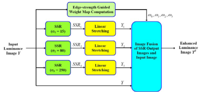
Fig. 1 Flow diagram of the proposed EGMSR approach
