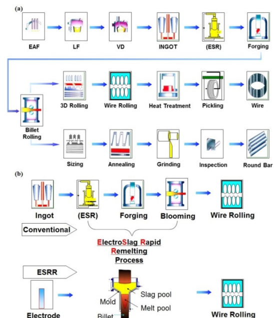
Fig. 1 Illustration of traditional (a) and ESRR (b) processes used for production of HSS products [5]
