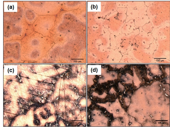
Fig. 8 Microstructure of AZ91D alloy aged at 200°C for various times of 10 min (a), 1 hr (b), 10 hrs (c), and 48 hrs (d), respectively
