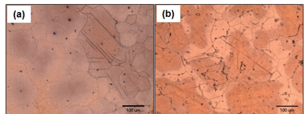
Fig. 4 Typical microstructure of AZ91D alloy (a) and nonflammable alloy (b) obtained after solid solution treatment followed by water quenching
