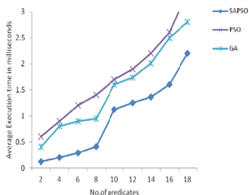
Fig. 4 Average Execution times (FOAF dataset)
