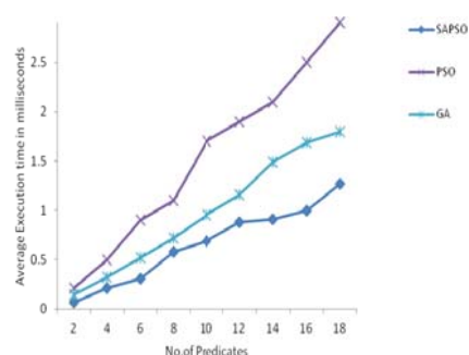
Fig. 5 Average Execution times (CIA World Factbook dataset)
