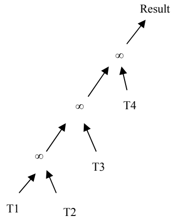
Fig. 1 A sample left deep tree
