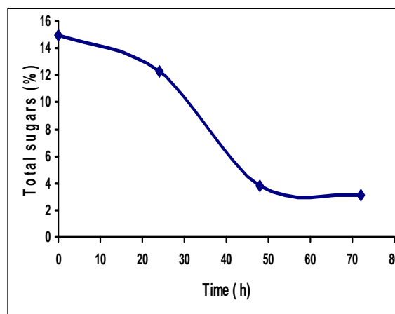
Fig. 4 Evolution of total sugars during the fermentation
