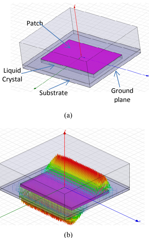
Fig. 1 Design configuration (a) Unit cell reflectarray design configuration and (b) E-field distribution for LC based unit cell
