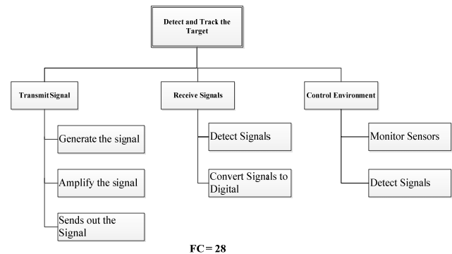
Fig. 1 The functional tree of an embedded system with its complexity
