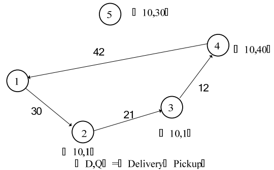
Fig. 3 Example of applying the route extraction algorithm
