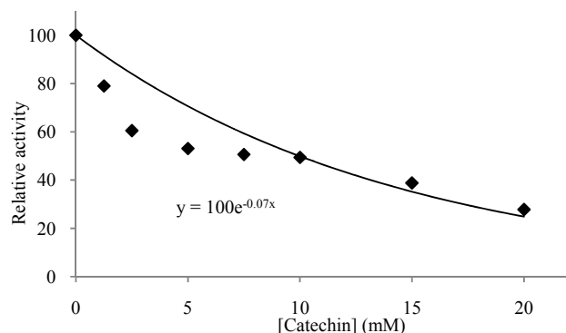
Fig. 1 [Catechin]-Activity (%) graphs for GST in the seven different catechin concentrations
