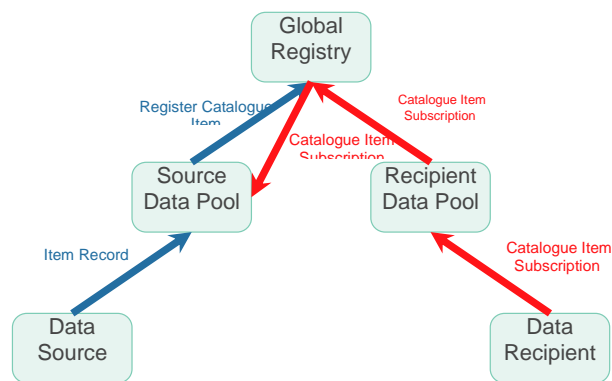
Fig. 6 GDSN Processes Enabled By GPC Without GPC These Processes Do Not Work [8]
