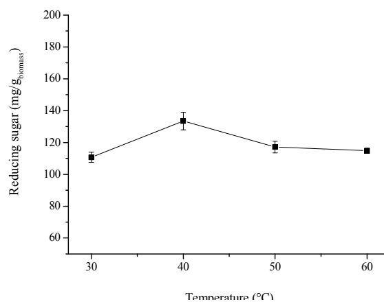
Fig. 4 The effect of temperature on saccharification of pre-treated T. suecica biomass Results represent the average value of 3 replicates
