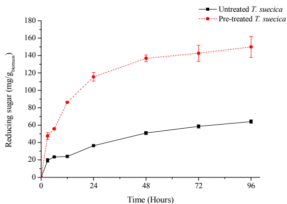
Fig. 1 Reducing sugar produced from enzymatic saccharification of untreated and alkaline pre-treated T. suecica biomass
