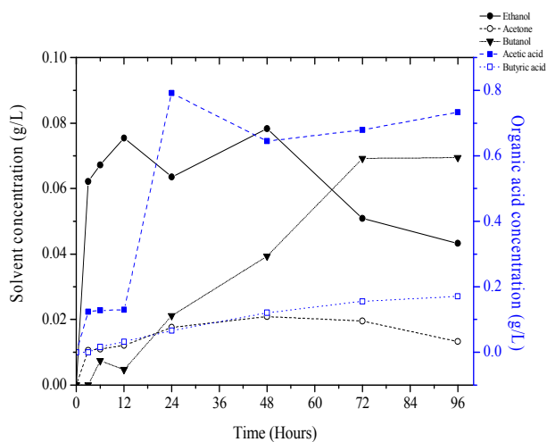
Fig. 7 ABE fermentation of hydrolysate enzymatic saccharification of alkaline pre-treated T. suecica biomass
