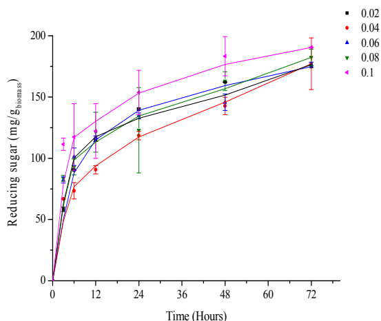
Fig. 6 The effect of enzyme to solid ratio ( [E]/[S] ) of pre-treated T.suecica biomass Results represent the average value of 3 replicates
