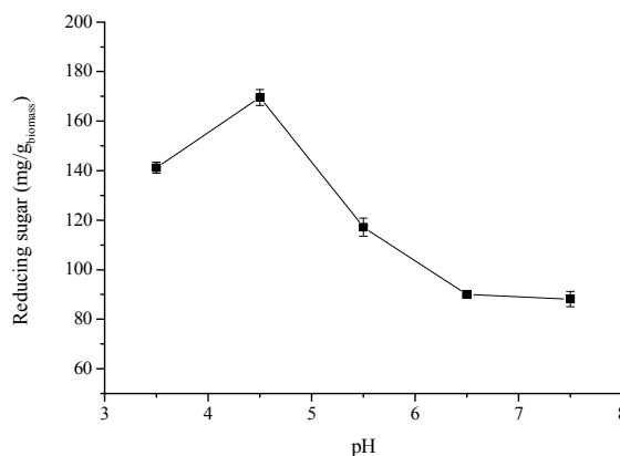
Fig. 5 The effect of pH on saccharification of pre-treated T. suecica biomass Results represent the average value of 3 replicates
