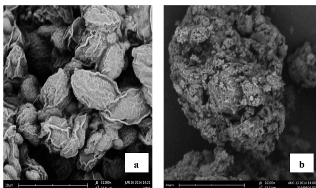
Fig. 2 SEM of T. suecica biomass (a) before alkaline pre-treatment, (b) after alkaline pre-treatment
