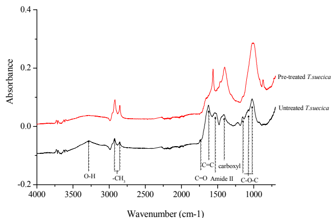
Fig. 3 FTIR spectra for raw and alkaline pre-treated microalgae biomass
