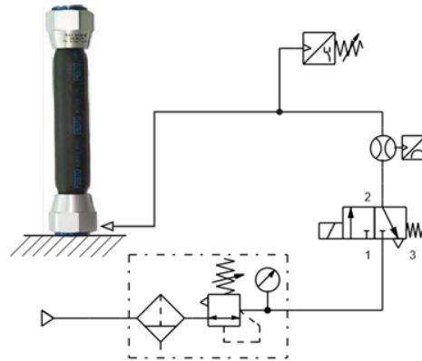
Fig. 12 Actuation diagram of the gripper system
