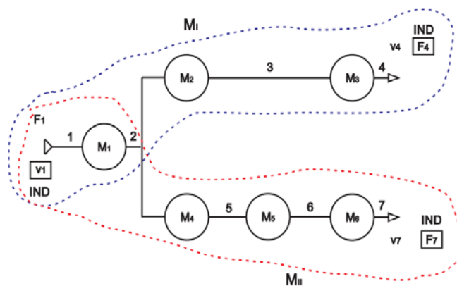
Fig. 4 Block diagram of the gripper system
