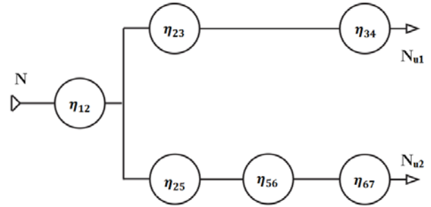
Fig. 5 Non-homogenous diagram of the aggregate with two parallel-connected mechanisms
