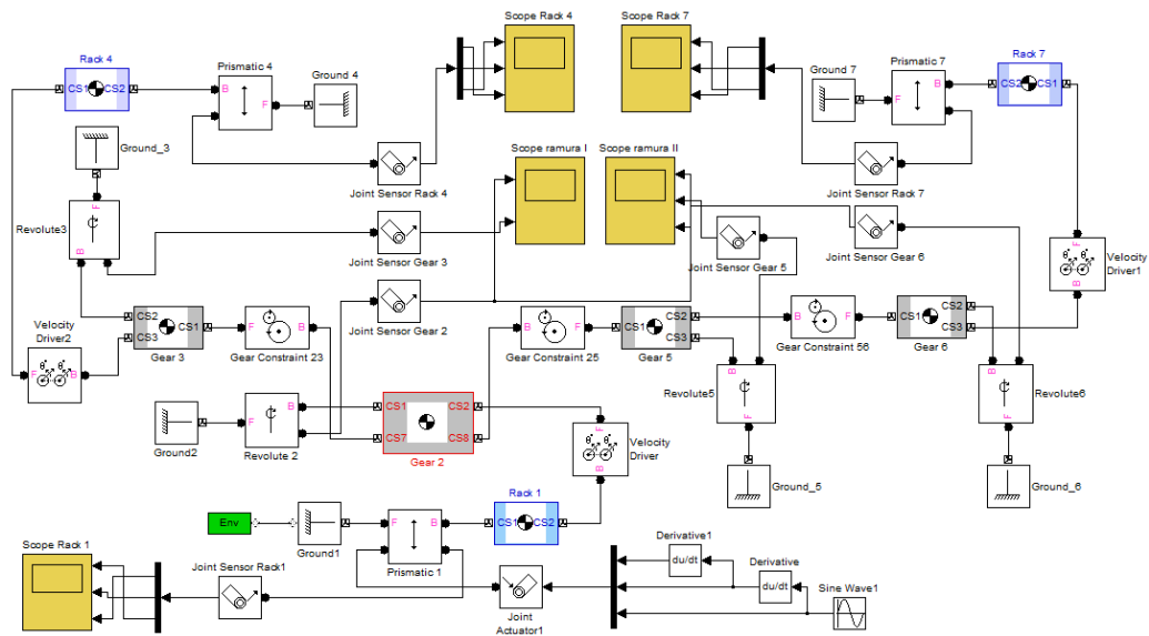
Fig. 9 Functional model of the gripper system
