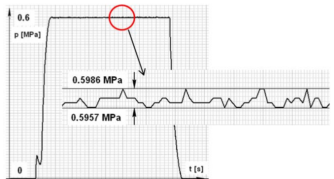
Fig. 13 Evolution of the pneumatic muscle feeding pressure
