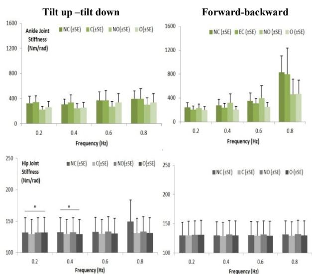
Fig. 3 Joint stiffness under four different frequency of perturbation ( \pm SE)(first row: ankle, second row: hip) with four different sensory limitations (NC=eyes closed with neck collar, C=eyes closed, NO=eyes-opened with neck collar, O=eyes opened)(*: p<0.05 )
